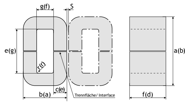
Angaben in (...) = IEC 60329 Bemaßung/ Descripton in (...) = IEC 60329 dimension
