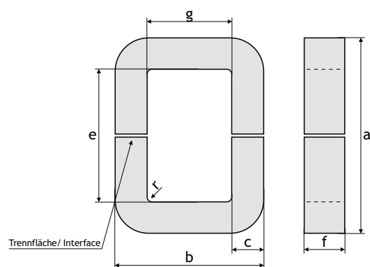
Angaben in (...) = IEC 60329 Bemaßung/ Descripton in (...) = IEC 60329 dimension
